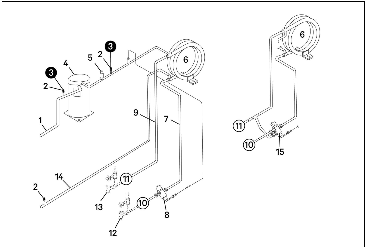
Figure 5.2 Valves and Connections for Water/Glycol Condensing Unit
