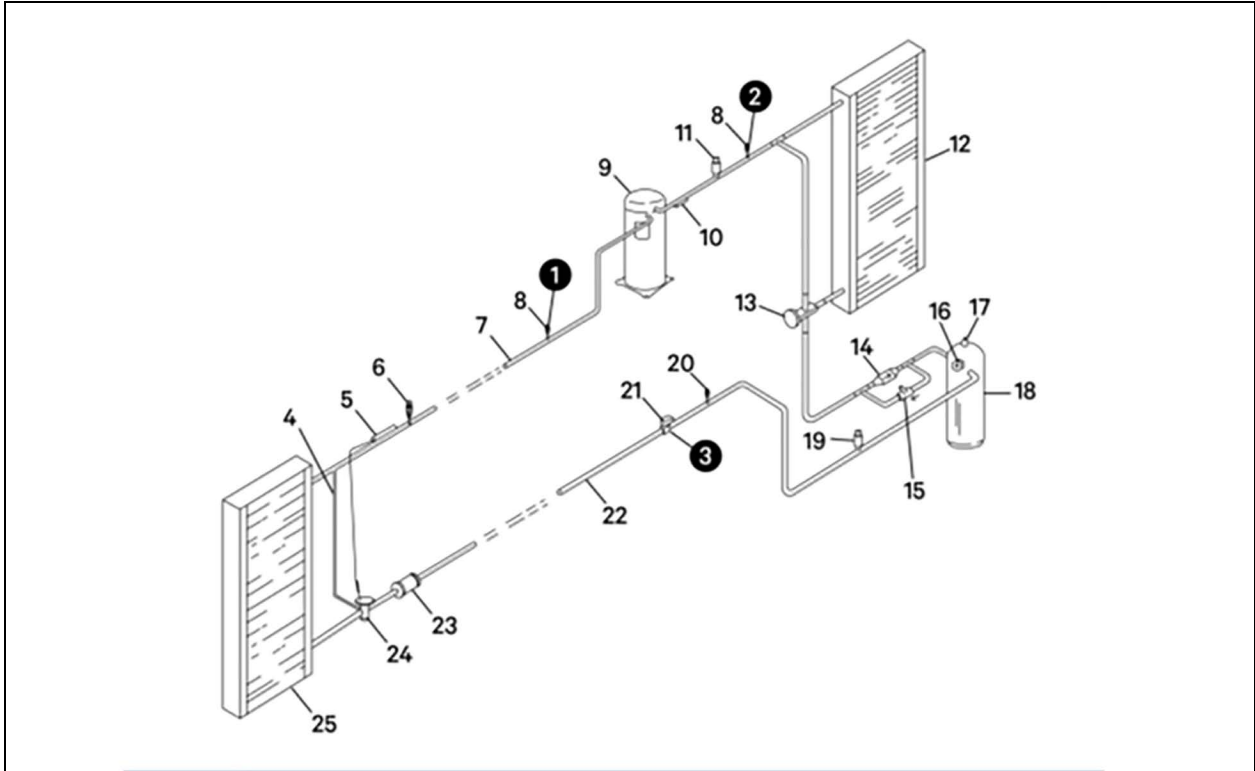
Figure 5.3 Valves and Connections for Air-cooled Condensing Unit
