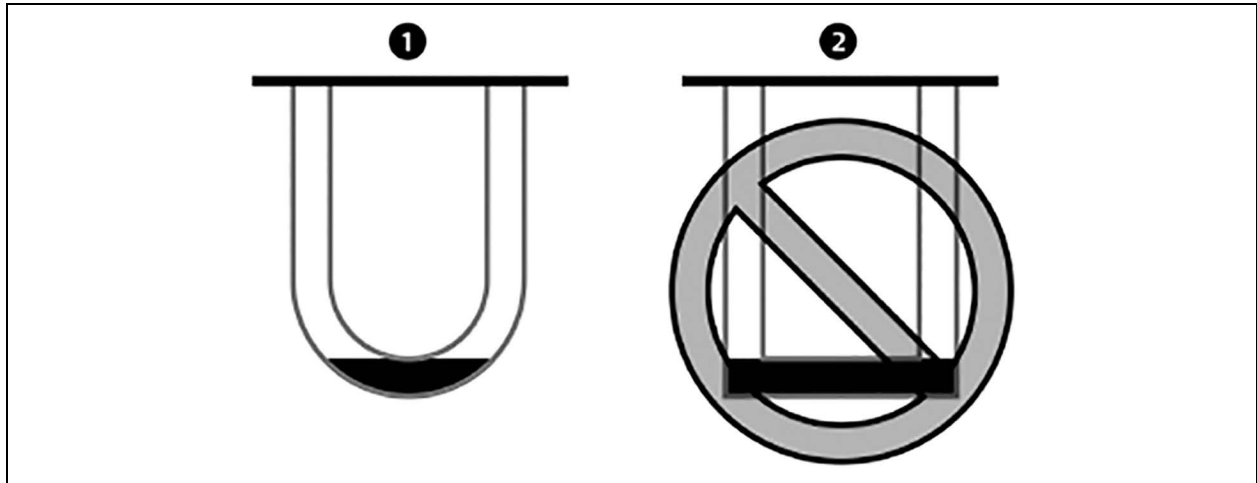
Figure 5.4 Standard Formed Tube Trap Versus Straight Tubes and Fittings Trap
