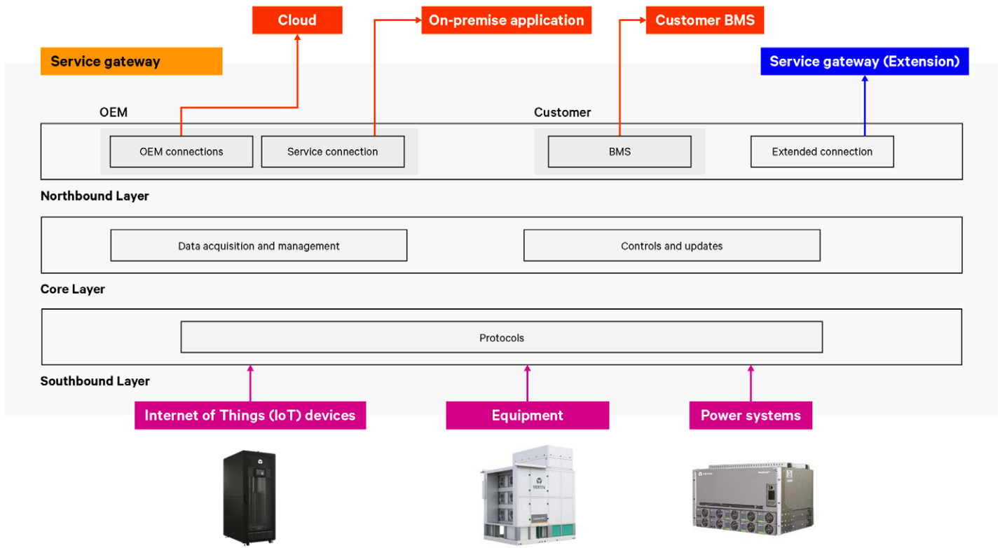
Figure 2. An advanced service gateway can provide options for collecting site data. The integrated system to the gateway creates a data pipeline from remote devices to on-prem machines for Vertiv teams' alert management, targeted maintenance interventions, increased product status confidence, and advanced asset management reporting.
