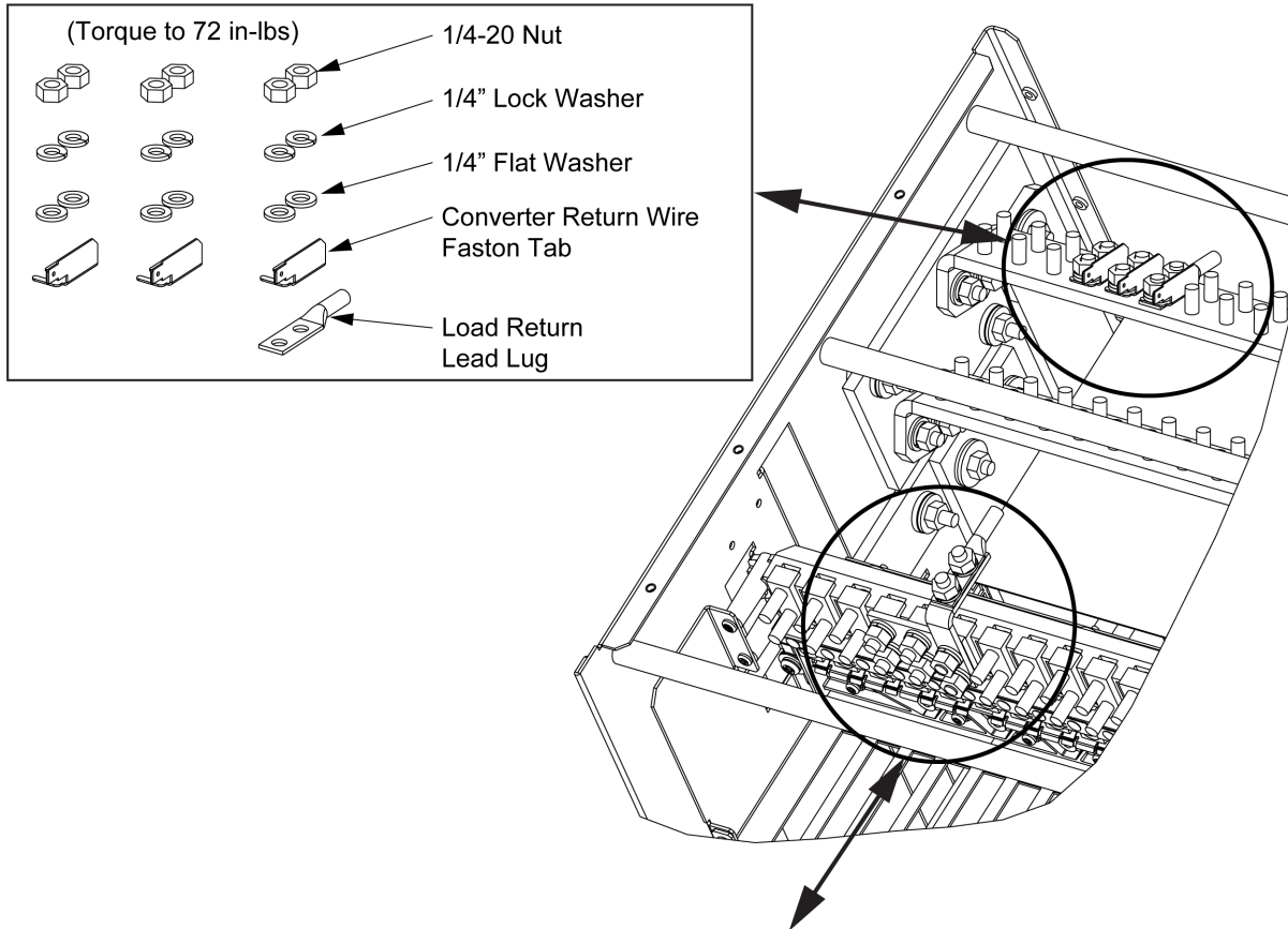
Figure 2.7 Connecting Converter Load and Load Return Cables, Installing Converter Return Wire Faston Tab, Installing Paralleling Busbar (P/N 60016097 or 545346) (cont'd from previous page)
