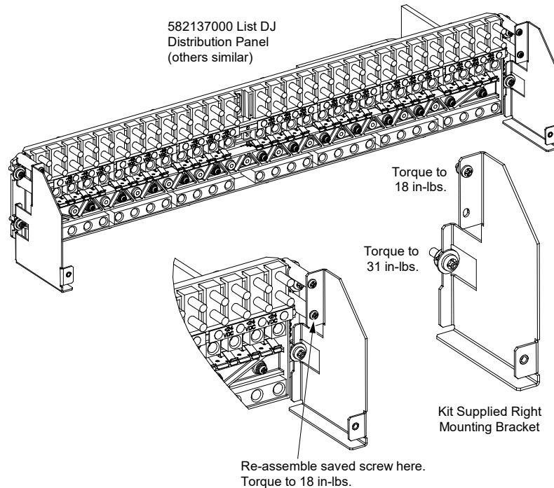
Figure 1.5 Install Right Side Mounting Bracket
