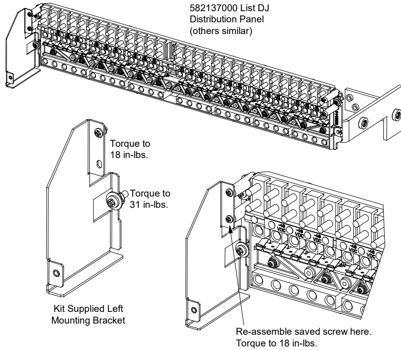
Figure 1.4 Install Left Side Mounting Bracket
