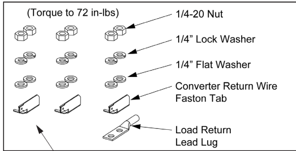
Figure 2.15 Connecting Converter Load and Load Return Cables, Installing Converter Return Wire Faston Tab, Installing Paralleling Busbar (P/N 60016097 or 545346) (cont'd from previous page)
