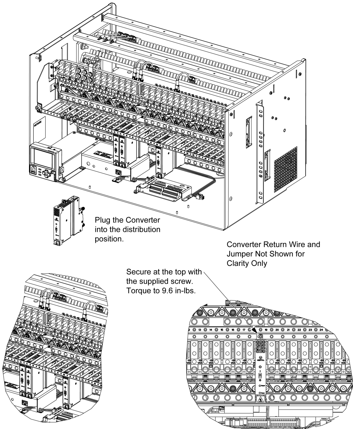
Figure 2.14 Installing Converter
