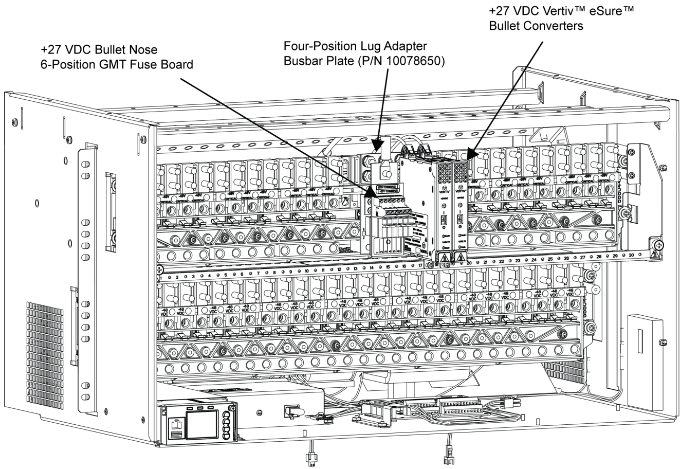
Figure 2.19 Installed +27 VDC Vertiv™ eSure™ Bullet Converters and +27 VDC Bullet Nose 6-Position GMT Fuse Board
