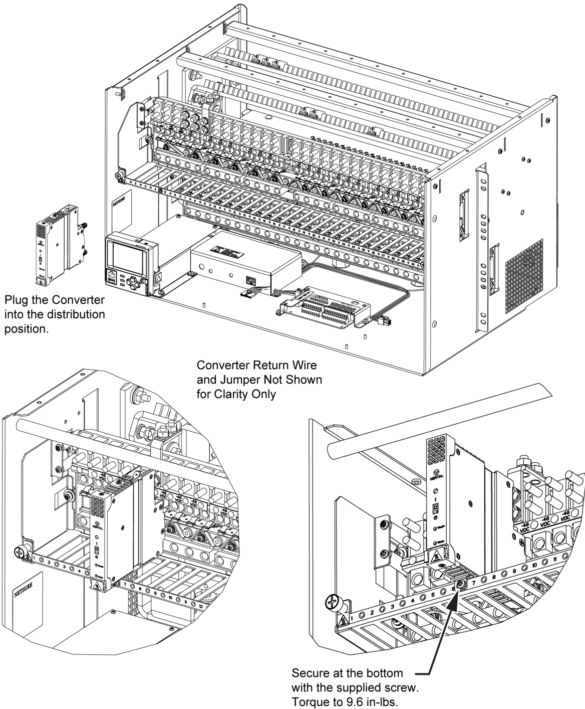
Figure 2.5 Installing Converter
