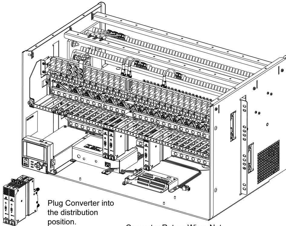
Figure 2.18 Installing Converters
