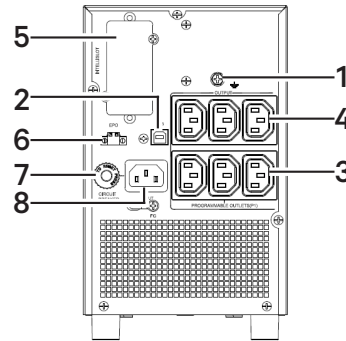
EDGE-1500IMT
